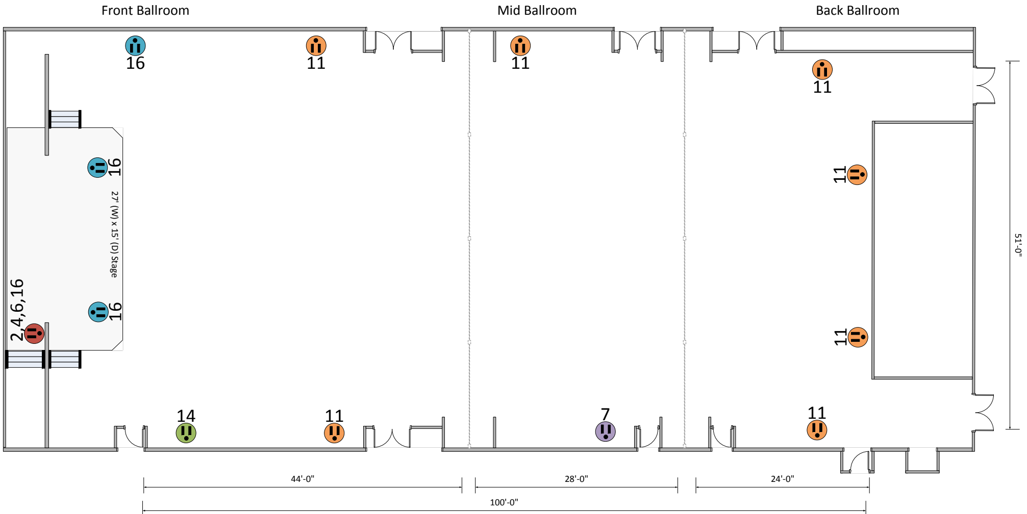
Hub Ballroom Electrical Layout Same Numbers = Same Circuit
